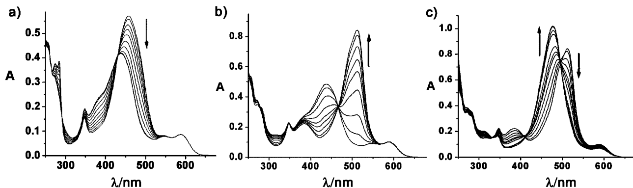
Fig. 2 The changes in UV-vis spectra of 1 recorded in CH_3CN ( 2.5 \times 10^{-5} M) after addition of: (a) 0, 0.1, 0.2, 0.3, 0.4, 0.5, 0.6, 0.7, 0.8, 0.9, 1.0 equiv of F^- ; (b) 1, 2, 3, 5, 7, 9, 15, 20, 30 equiv of F^- ; (c) 30, 40, 50, 60, 70, 80, 100, 125, 150, 175, 200 equiv of F^- .
