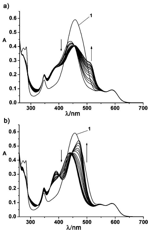
Fig. 3 The changes in UV-vis spectra of 1 recorded in \text{CH}_3\text{CN} ( 2.5 \times 10^{-5} M) after addition of (a) 0, 10, 20, 30, 40, 50, 60, 70, 80, 100, 120, 140, 160, 180, 200 equiv of \text{AcO}^- ; (b) 0, 1, 2, 3, 4, 5, 10, 15, 20, 30, 40, 50, 75, 100, 200 equiv of \text{H}_2\text{PO}_4^- .
