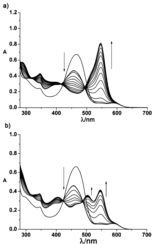
Fig. 6 The changes in UV-vis spectra of 3 recorded in CH_3CN ( 2.5 \times 10^{-5} M) after addition of (a) 0, 0.6, 0.8, 1, 1.2, 1.4, 1.6, 1.8, 2, 4, 6, 8, 10, 15, 20, 50, 100 equiv of AcO^- ; (b) 0, 1, 2, 4, 6, 8, 10, 15, 20, 30, 40, 60, 80, 100 equiv of H_2PO_4^- .
