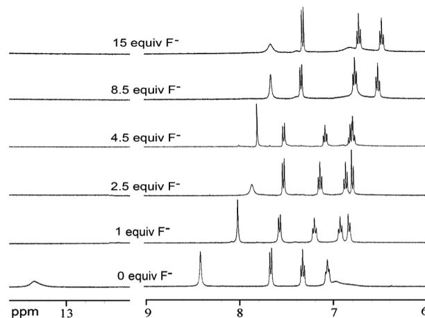
Fig. 4 ^1\text{H} NMR spectra of 1 ( 1.0 \times 10^{-2} M) in \text{DMSO}-d_6 upon addition of various quantities of tetrabutylammonium fluoride.
