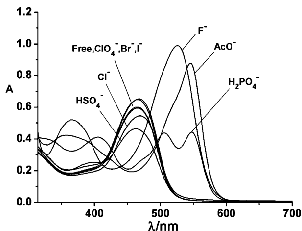
Fig. 5 UV-vis spectra of 3 recorded in CH_3CN ( 2.5 \times 10^{-5} M) after addition of 25 equiv of various anions (none, F^- , AcO^- , Cl^- , Br^- , I^- , HSO_4^- , ClO_4^- , H_2PO_4^- ).
