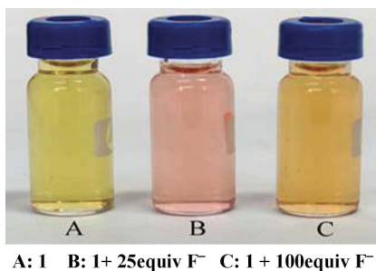
Fig. 1 Color changes of 1 ( 2.5 \times 10^{-5} M in CH_3CN ) upon addition of 0, 25, 100 equiv of F^- .
