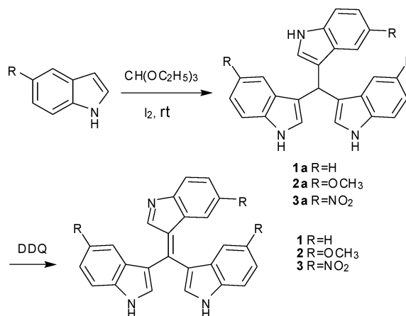
Scheme 1 Synthesis of compounds 1–3 .
